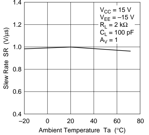
Slew Rate vs. Ambient Temperature
